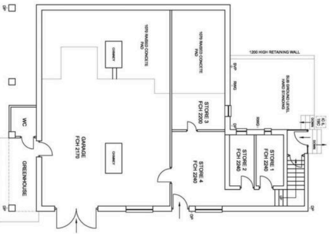
EXISTING BASEMENT SCALE 1:100
